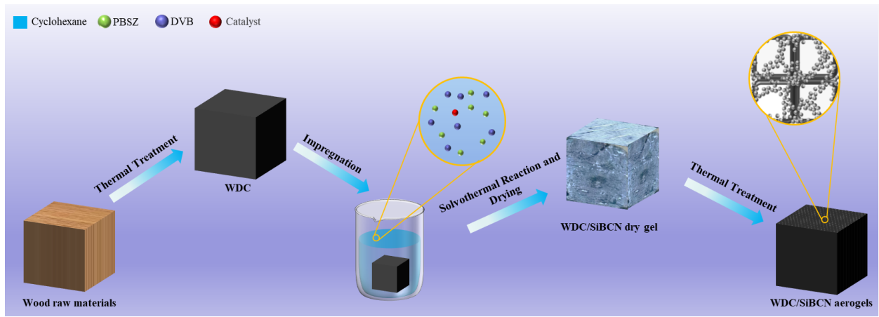
Figure 1: Preparation steps of WDC/SiBCN aerogel composites.
