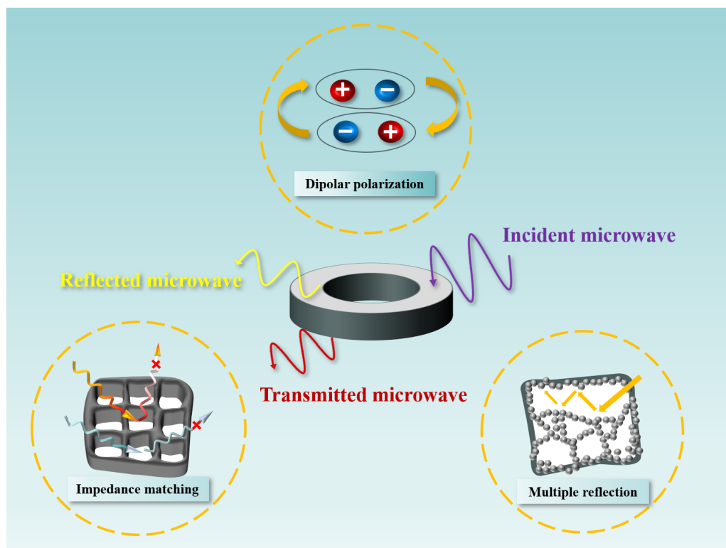
Figure 8: Microwave absorption mechanism.
