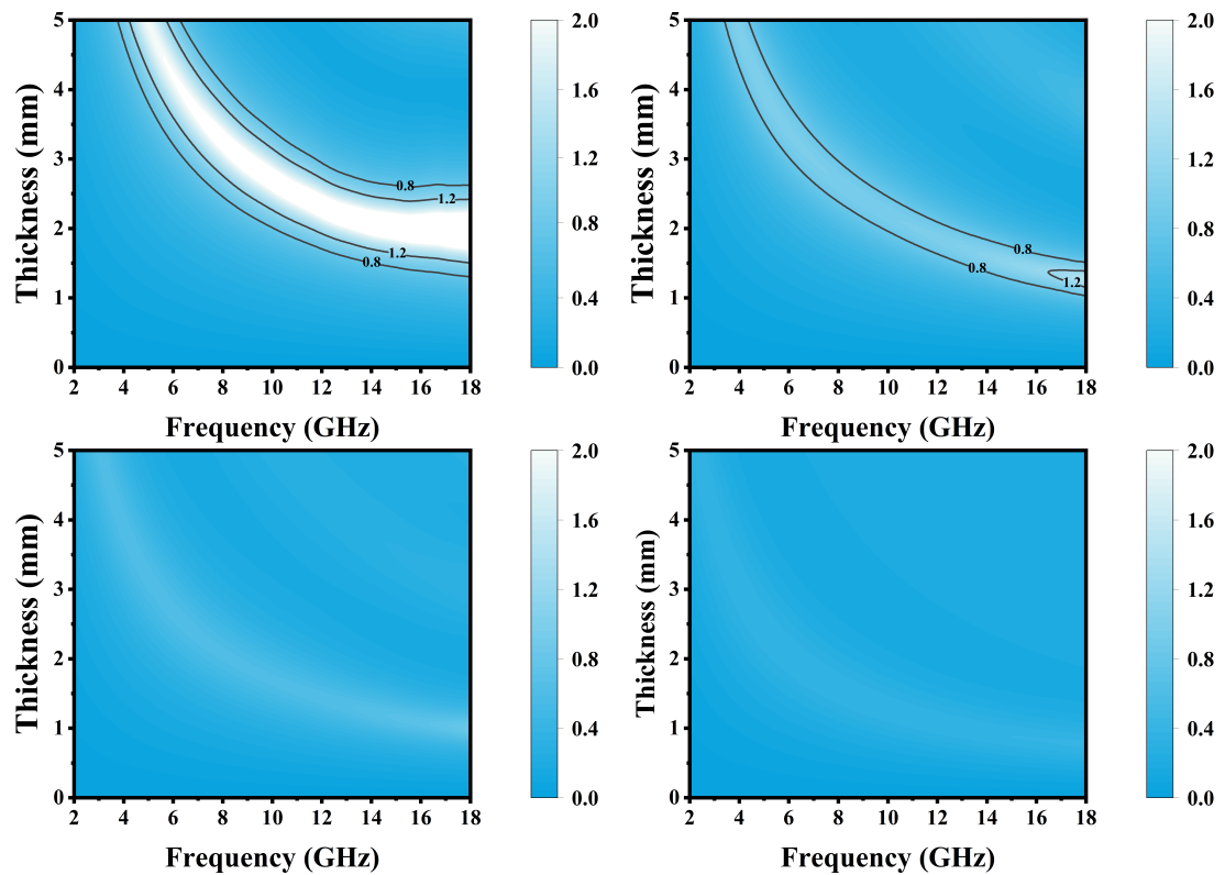
Figure 6: Z of the prepared composites:(a) WDC;(b) WDC/SiBCN-5;(c) WDC/SiBCN-10;(d) WDC/SiBCN-15.
