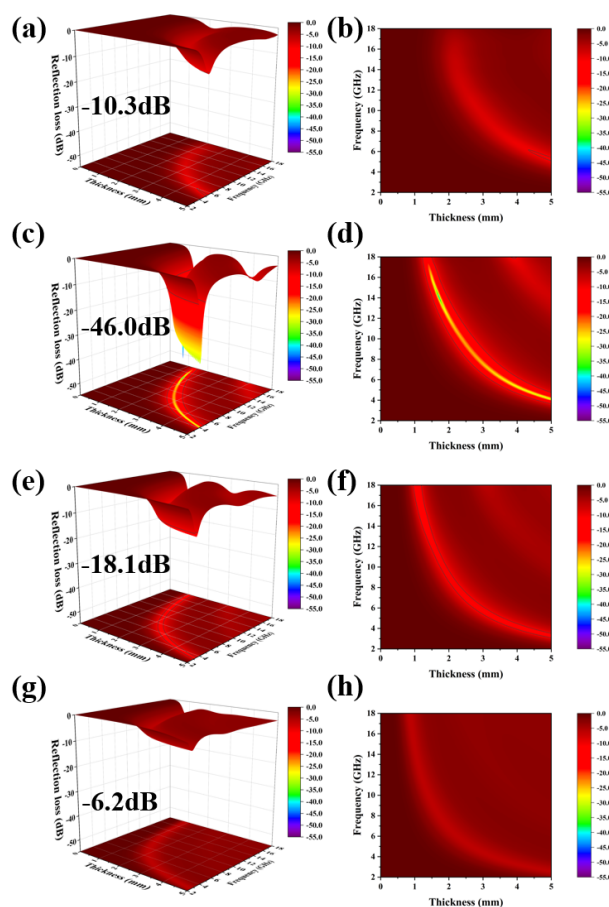
Figure 4: RL images and curves of WDC and WDC/SiBCN aerogel composites at different frequencies; (a, b) WDC; (c, d) WDC/SiBCN-5; (e, f) WDC/SiBCN-10; (g, h) WDC/SiBCN-15.
